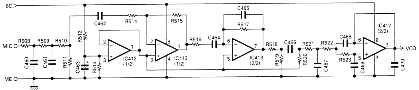
Fig. 15 Microphone amplifier circuit
