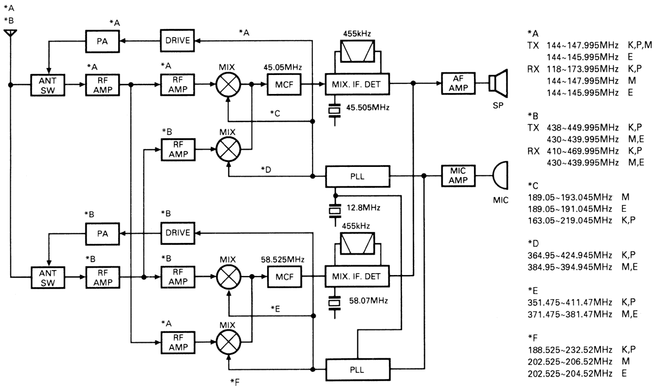
Fig.1 Frequency configuration
