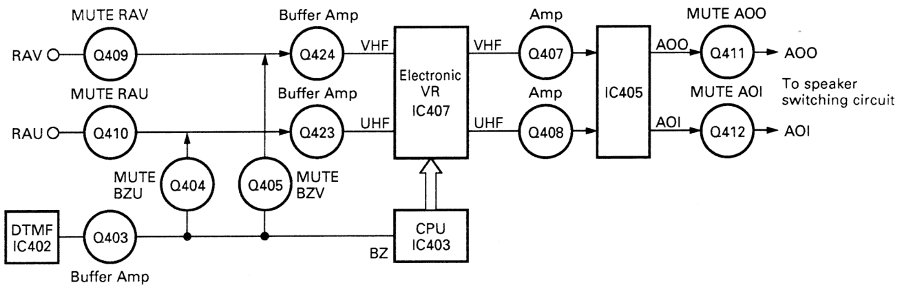
Fig. 7 AF signal system block diagram
