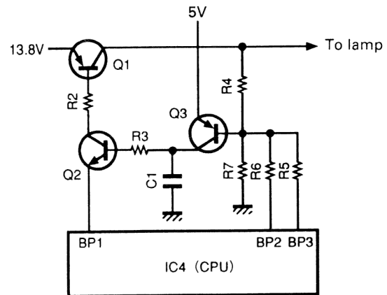
Fig. 17 Dimmer circuit
