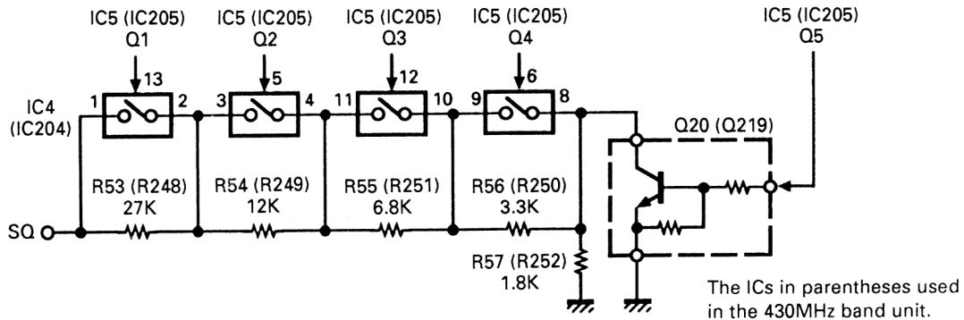
Fig. 4 Squelch circuit
